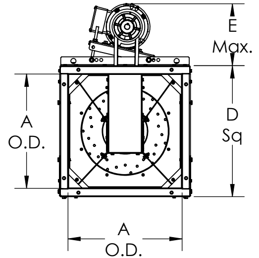
DISCHARGE VIEW
