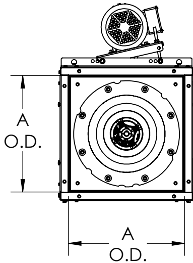
INLET VIEW
